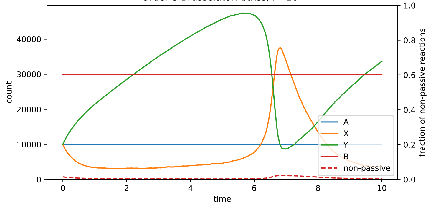
Order-3 Brusselator: batss, n=10^4
